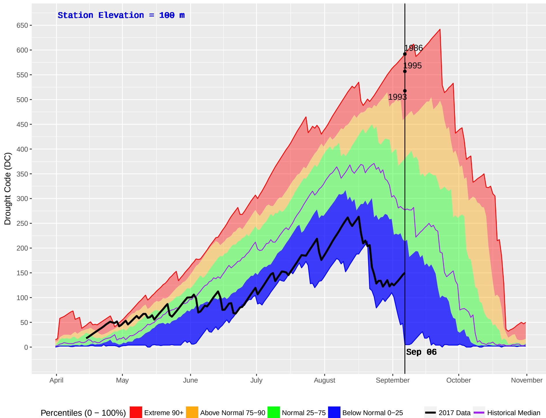
HONNA (93) : Historical (1986–2016) and Current (2017) Noon Drought Code (DC)
