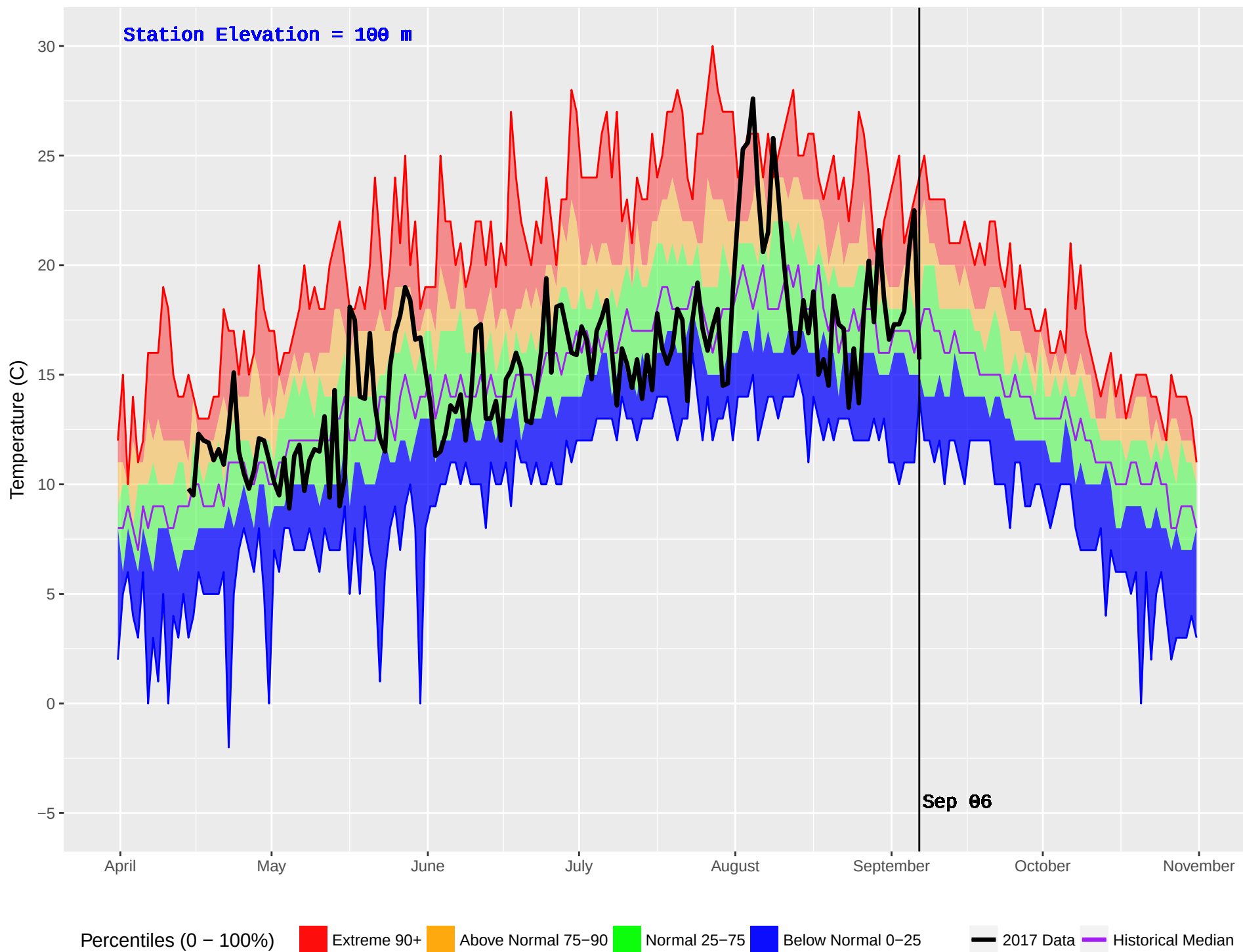
HONNA (93) : Historical (1986–2016) and Current (2017) Noon Temperature
