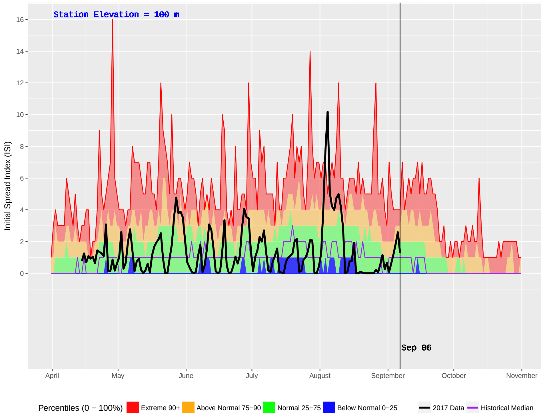
HONNA (93) : Historical (1986–2016) and Current (2017) Noon Initial Spread Index (ISI)
